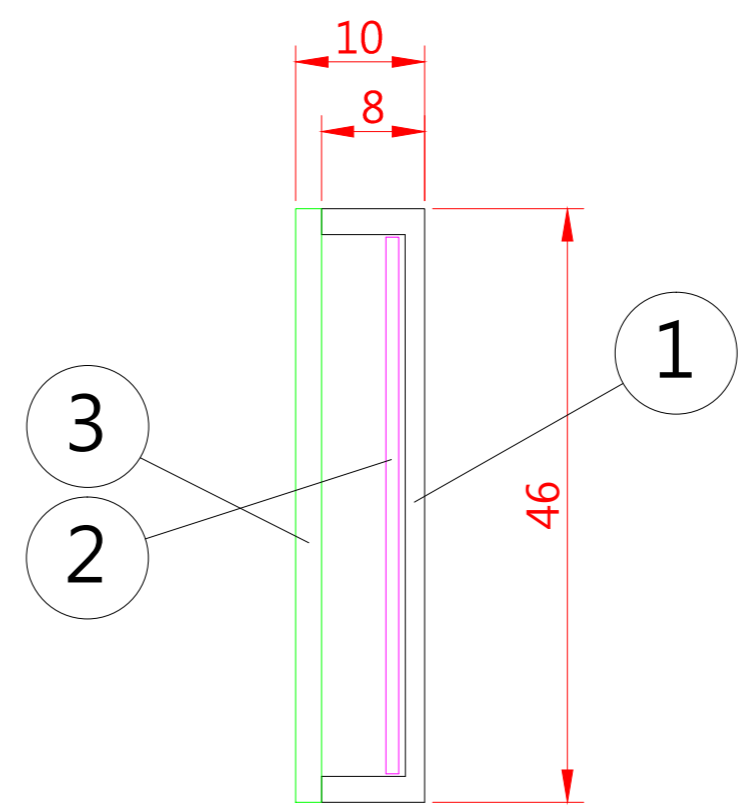
SECTION B-B'
