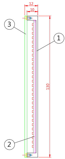
SECTION B-B'
