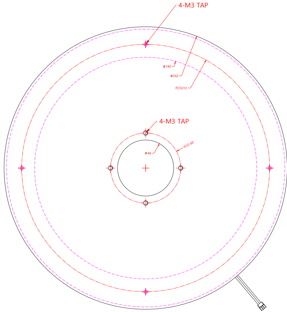
[ TOP VIEW ]
