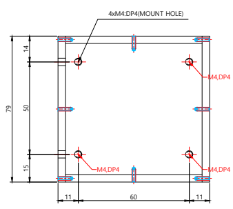
LEFT VIEW
